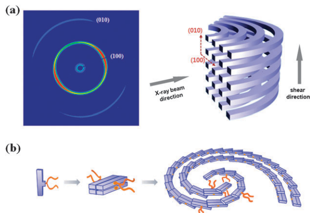
Fig. 3 (a) 2D-SAXS pattern obtained from the sheared sample of 1 at 25 °C. The X-ray pattern was recorded on the sample along a direction perpendicular to the shear. The diffraction pattern shows {100}, {010} reflections. (b) Schematic representation of the packing model of 1 .
