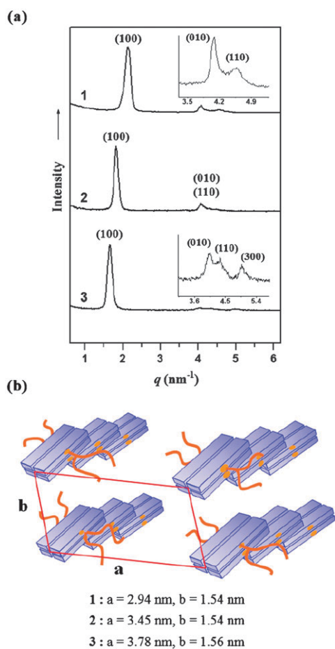
Fig. 2 (a) SAXS patterns of 1 – 3 plotted against q ( = 4\pi \sin \theta \lambda^{-1} ) (Inset: magnified SAXS reflections in the range of q = 3.5 – 5.5 \text{ nm}^{-1} ). (b) Schematic representation of a 2D rectangular structure.
