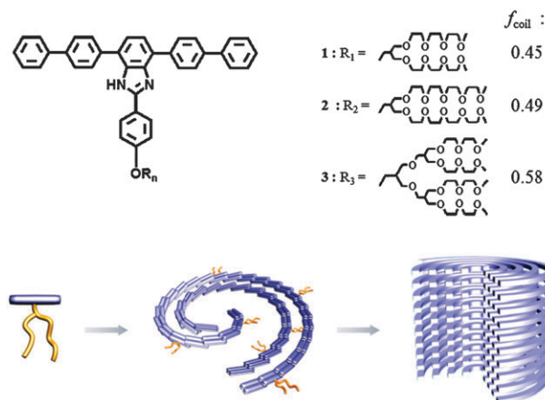
Fig. 1 Schematic representation of spiral columns and molecular structure of 1–3 .
